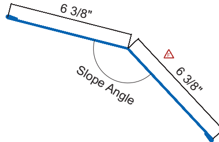
Gambrel Flashing
