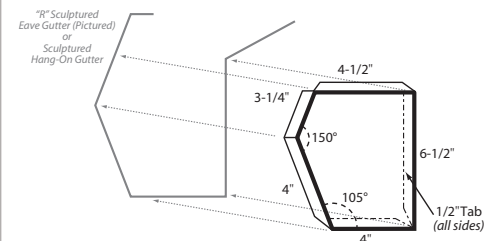
Sculptured Gutter End Cap
