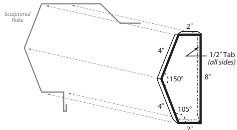
Sculptured Rake End Cap
