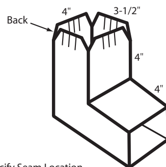
Downspout Elbow DS35A1: 45° angle (w 45° & 95° Elbow) DS35A2: 95° angle
