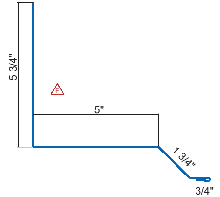
Sidewall/Parapet Rake Trim
