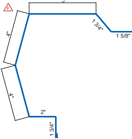
Sculptured Rake Trim
