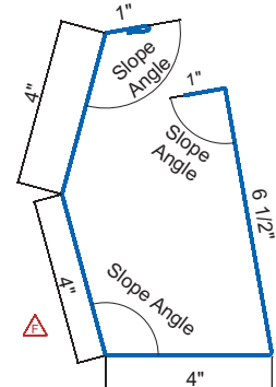
Sculptured Hang-On Gutter
